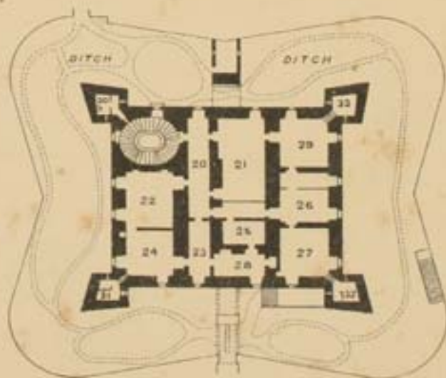
BASEMENT PLAN.
