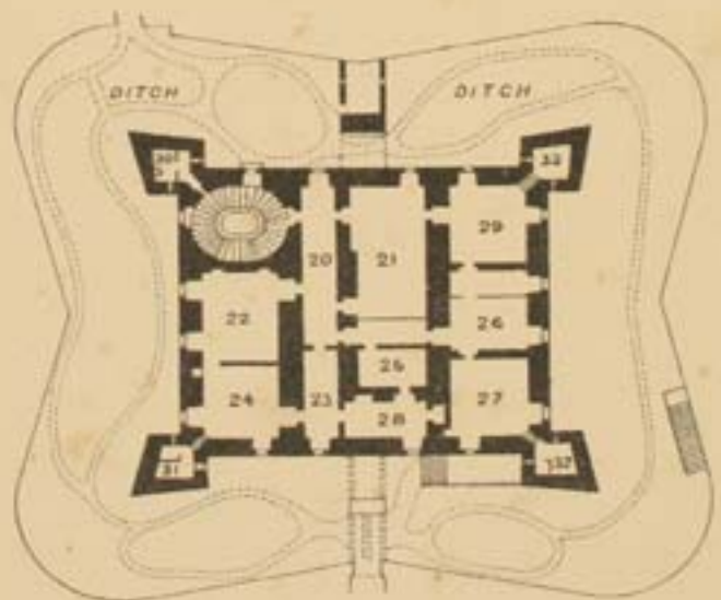
BASEMENT PLAN.
