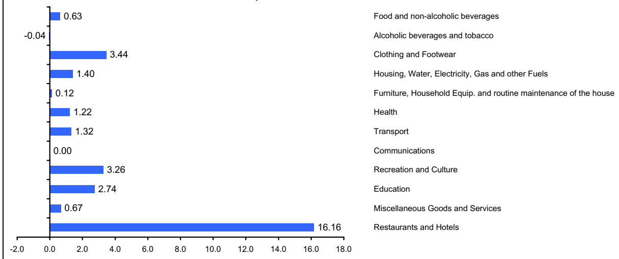
Chart 4. HICP percentage points change: April 2006 over March 2006
