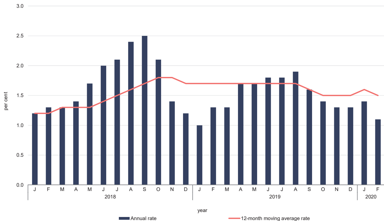
Chart 1. Inflation rates
