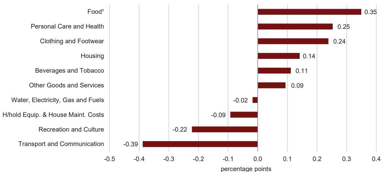
Chart 3. Contribution to the annual inflation rate by the 10 main groups: August 2020
