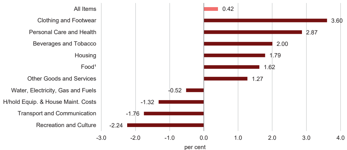
Chart 2. Annual inflation rates by the 10 main groups: August 2020
